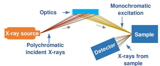
Figure 1. MXRF Technology
